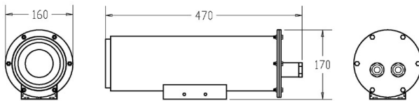
Type 1A face view Type 1A side view Type 1A back view
