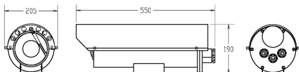
Type C face view Type C side view Type C back view
