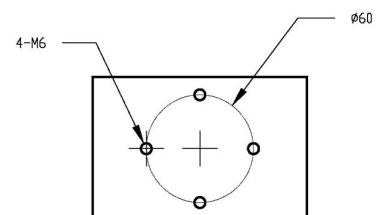
Bottom mount hole
