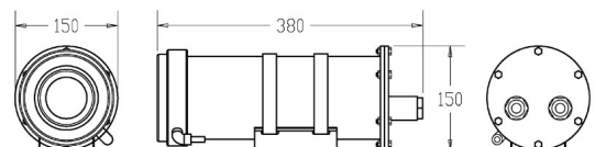
Type 2B face view Type 2B side view Type 2B back view
