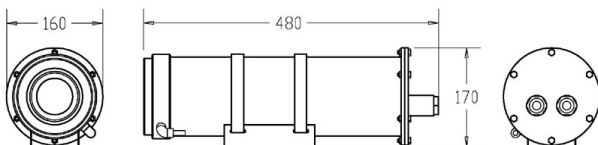
Type 2A face view Type 2A side view Type 2A back view
